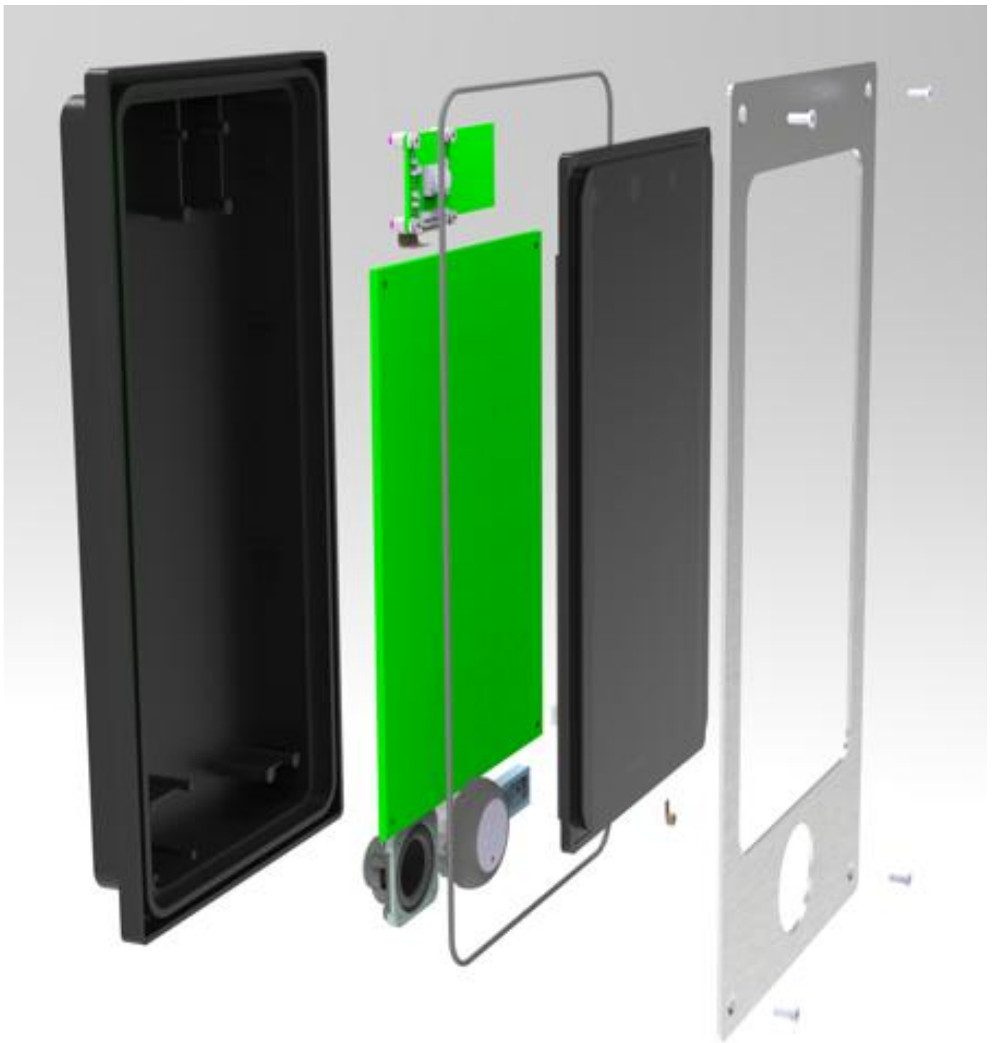
Architecture interne (2)
